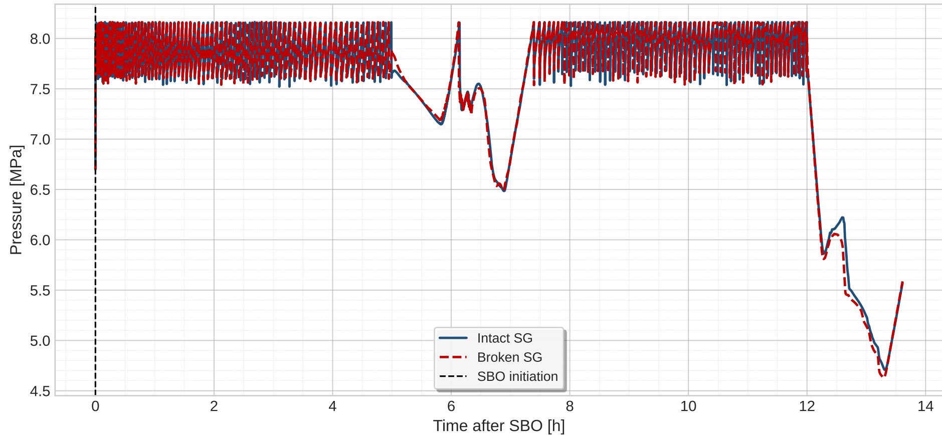
No SG Depressurization - Secondary Pressure (SG Cooldown)
